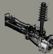
MacPherson Strut
